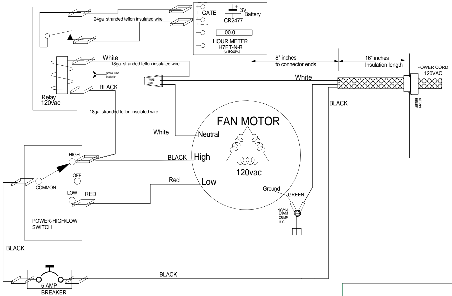
MICROCON AS WIRING DIAGRAM Motor and Air Flow Switch
